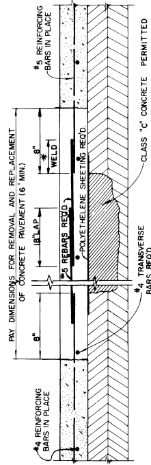
SECTIONAL VIEW (SHOWING REPLACED AREA)
