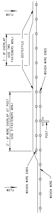
PLAN VIEW
