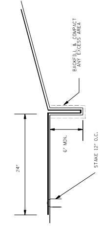
DETAIL OF BOTTOM TRENCH
