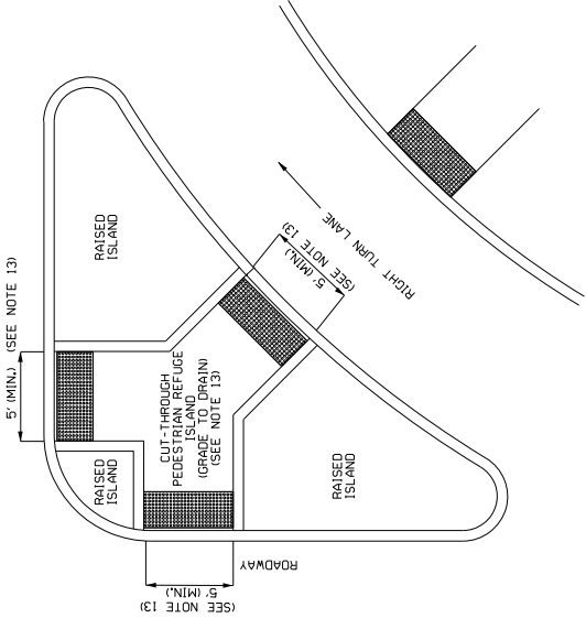
CURB RAMP CONFIGURATION: TYPE I NOT RECOMMENDED
