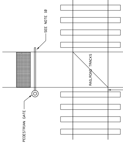
DETECTABLE WARNINGS AT BLENDED TRANSITION
