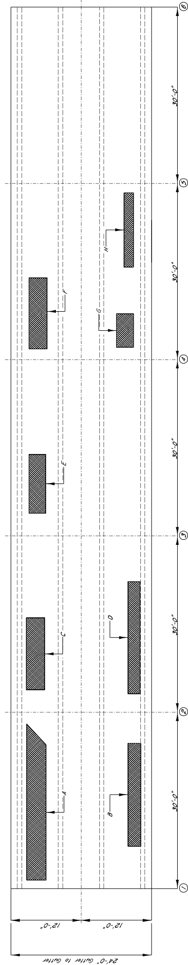
PLAN OF SPAN BRIDGE NAME: 39.6 Showing areas of bridge deck to be repaired
