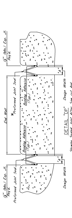
DETAIL "E" Showing Joint After Saw cut And Repair With Epoxy Matrix
