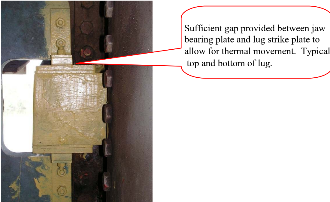
Photo No. 6 Fixed unit lug at Bascule Girder G4 (7/14/09).
