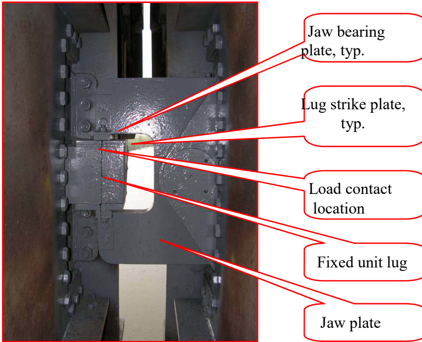
Photo No. 5 Jaw plate to fixed unit lug at Bascule Girder G1 (7/14/09).
