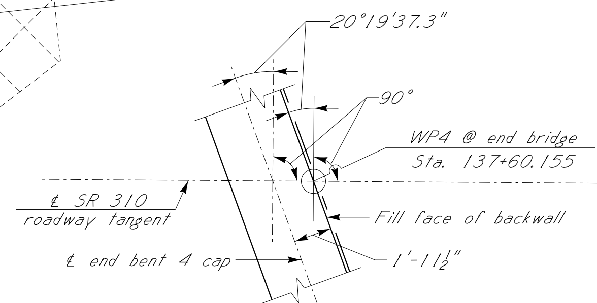
BRIDGE END DETAIL Scale: 1" = 5'-0"
