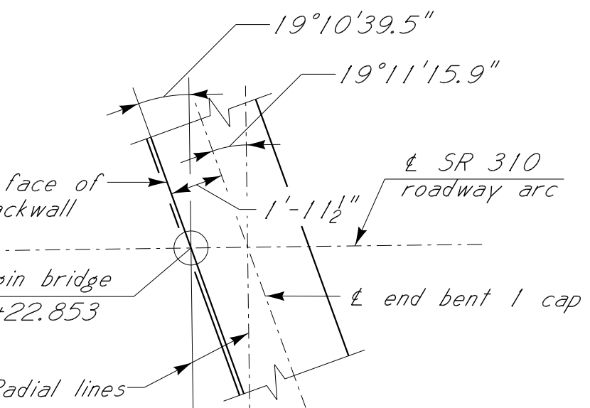
BRIDGE BEGIN DETAIL Scale: 1" = 5'-0"
