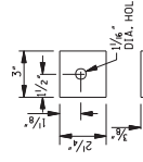
BRACKET
