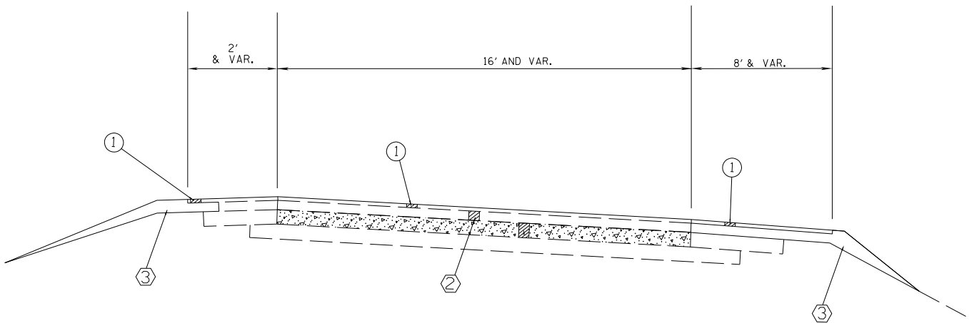
TYPICAL SECTION INTERCHANGE RAMPS
