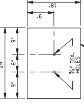
SOIL PLATE
