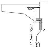
ELEVATION AT END OF SPAN
