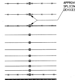
SPlicing DETAILS BETWEEN POSTS
