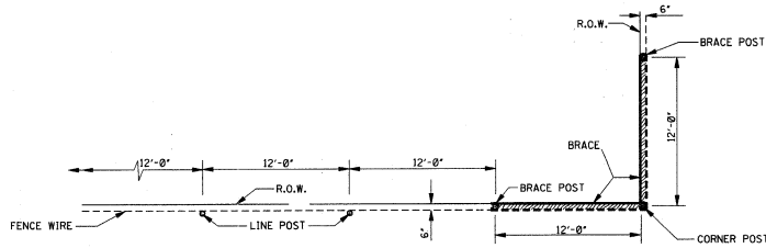
PLAN SHOWING PLACEMENT OF FENCE ALONG RIGHT OF WAY
