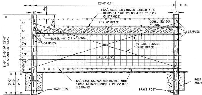
DETAIL OF BRACE BAY
