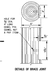
DETAILS OF BRACE JOINT
