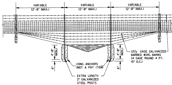
CROSSING TYPE III
