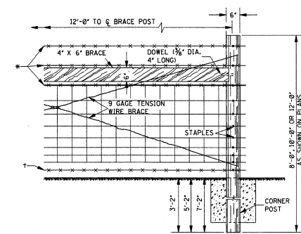
DETAIL OF CORNER BRACE
