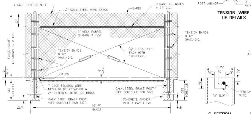
INTERMEDIATE BRACE BAY
