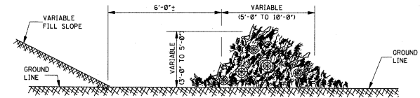
SIDE ELEVATION
