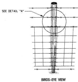
DETAILS OF LINE FENCE AND LINE POSTS
