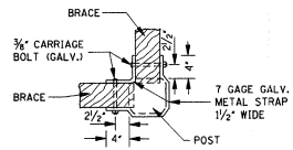
DETAIL OF FASTENER BRACE TO BRACE AT CORNER
