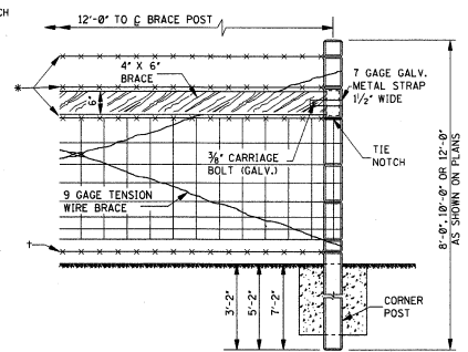
DETAIL OF CORNER BRACE
