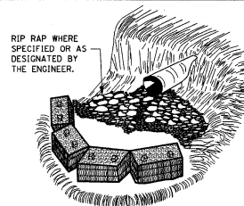
CULVERT
