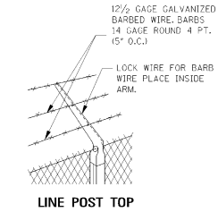
LINE POST TOP (VERTICAL ARMS WHEN DESIRED)
