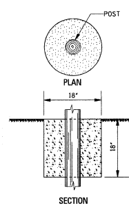
POST ANCHOR DETAILS
