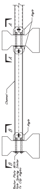
TEMPORARY STEEL BRACING DETAILS AASHTO Type-1A, 2, 3, 4, 5, 6, 7, 8, & 9 Beams
