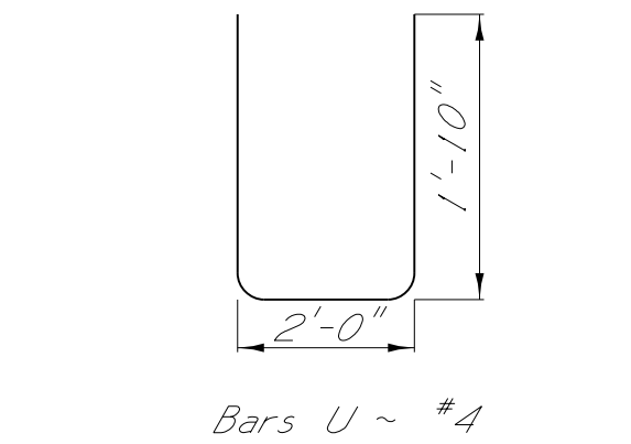
BAR BENDING DETAILS All dimensions are out to out
