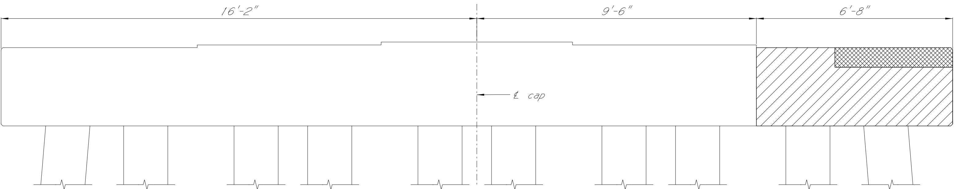
ELEVATION OF BENT Showing Epoxy Mortar Locations at Bent No. 4, Span No. 3
