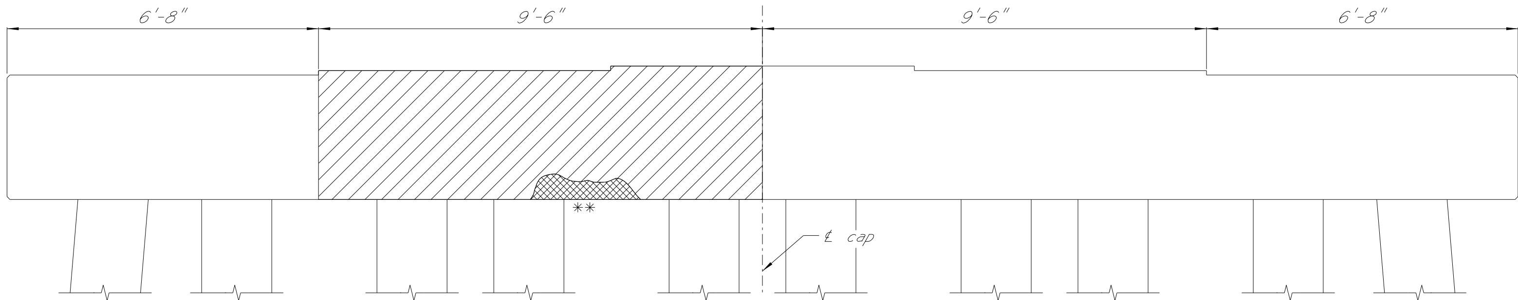
ELEVATION OF BENT Showing Epoxy Repair and FRP Wrap at Bent No. 6, Span No. 5
