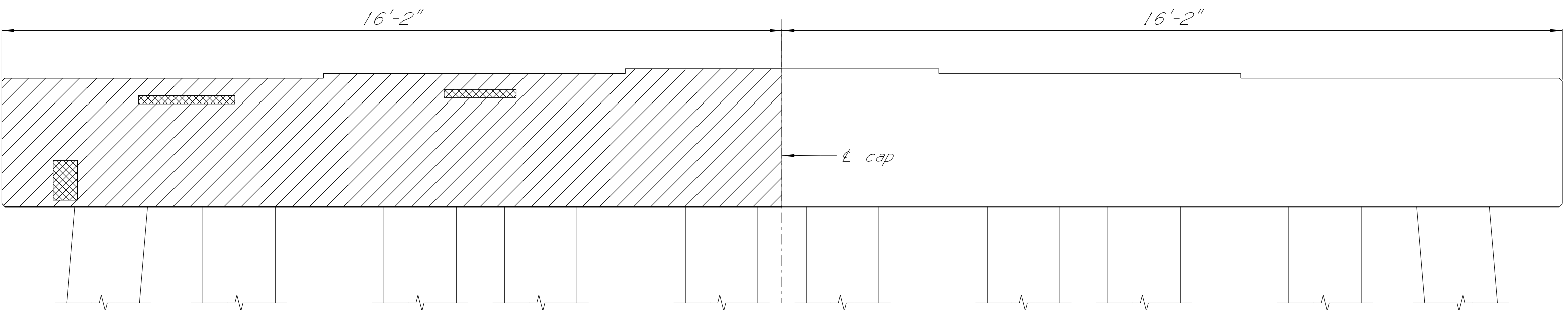
ELEVATION OF BENT Showing Epoxy Mortar Locations at Bent No. 2, Span No. 1
