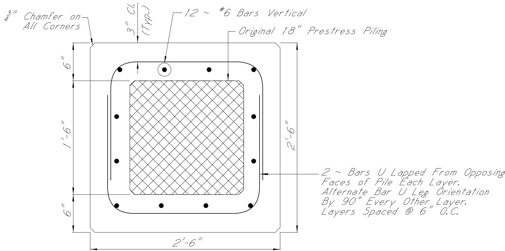
SECTION A-A Dimensions are out to out
