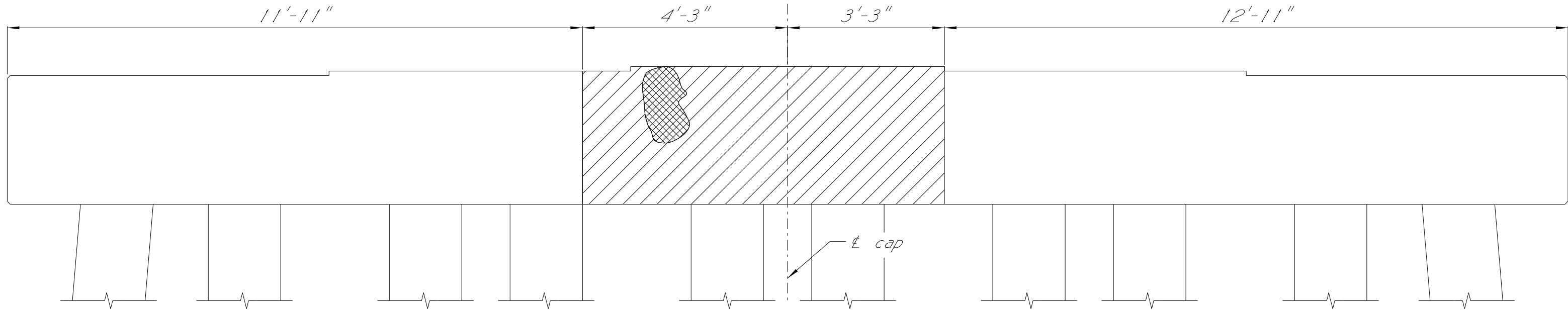
ELEVATION OF BENT Showing Epoxy Repair and FRP Wrap at Bent No. 10, Span No. 9
