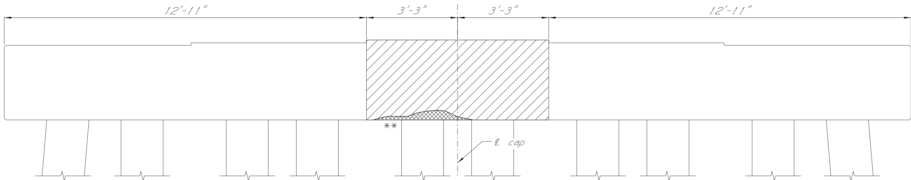
ELEVATION OF BENT Showing Epoxy Repair and FRP Wrap at Bent No. 7, Span No. 6
