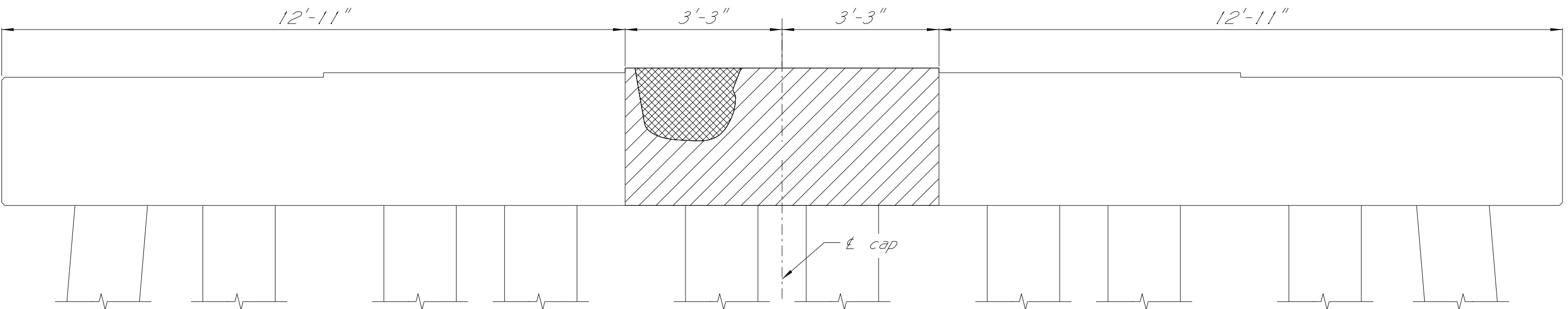
ELEVATION OF BENT Showing Epoxy Repair and FRP Wrap at Bent No. 3, Span No. 2
