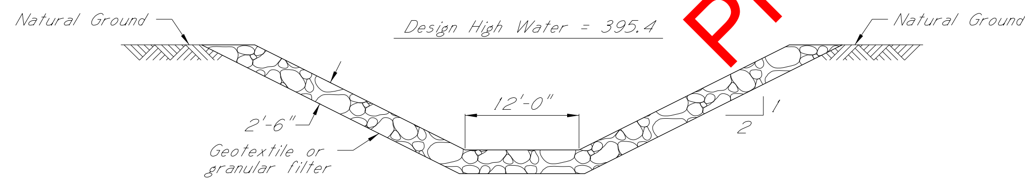
CROSS SECTION OF BANK STABILIZATION
