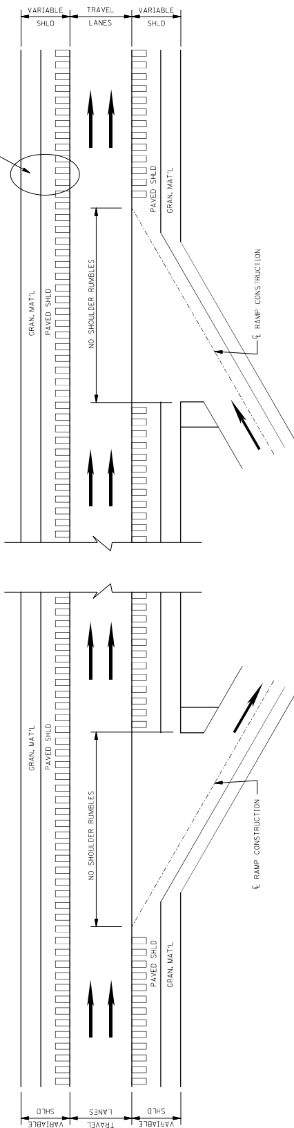
PLAN NOT TO SCALE DETAILS OF RUMBLE STRIPES
