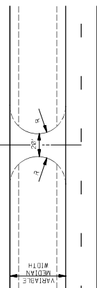
DETAIL OF TEMPORARY CROSSOVER NOTE: P = 60.5 MEDIAN #13110
