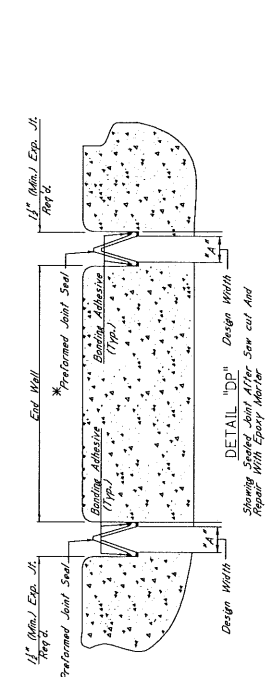
DETAIL 'D'
