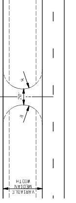
DETAIL OF TEMPORARY CROSSOVER NOTE: P = 60 ft. MEDIAN W20-10'
