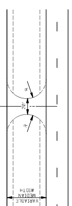
DETAIL OF TEMPORARY CROSSOVER NOTE: R = 60\"/>
