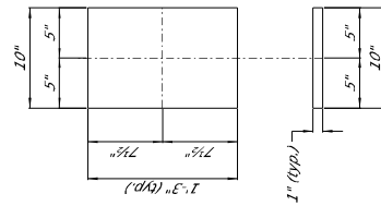
NEOPRENE PAD DETAILS
