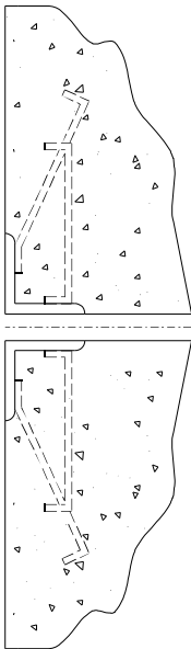
TYPICAL SECTION AT EXISTING JOINT - BENTS 2 - 4
