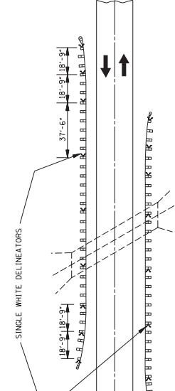
ROADSIDE OBSTACLE INSTALLATION—LENGTH 250' OR LESS (TWO-WAY TRAFFIC)
