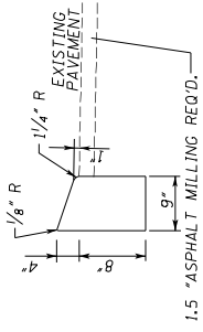
Type 2 Special Design Header Curb
