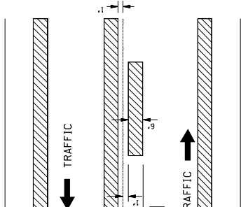
DETAIL "A" PLACEMENTS WITHOUT RUMBLE STRIPS
