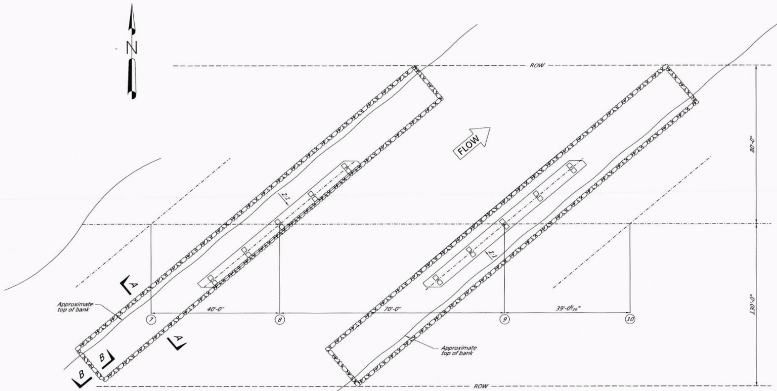
RIPRAP PLACEMENT PLAN Showing limits of riprap placement (BR 7.1)
