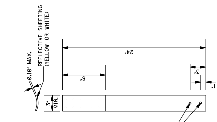
DETAIL OF FLEXIBLE GUARDRAIL DELINEATOR
