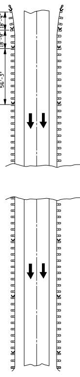
GRAPHIC SHOWING SPACINGS OF GUARDRAIL DELINEATORS AT SOME COMMONLY USED BRIDGE APPROACHES
