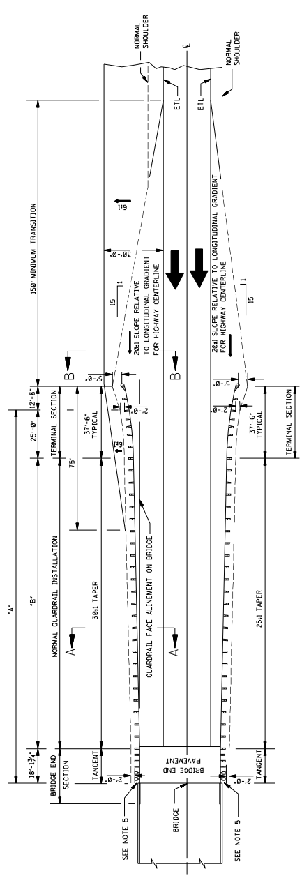
DIVIDED HIGHWAY WITH BARRIER INSIDE CLEAR ZONE OF OPPOSING TRAFFIC
