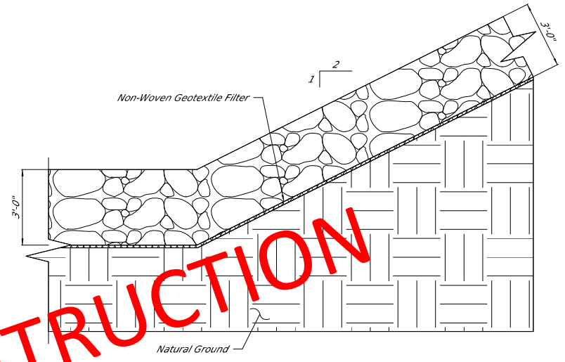
SECTION B-B Riprap Toe Detail Not to Scale
