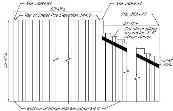
LAYOUT OF SHEET PILE Along \phi Roadway and Bridge
