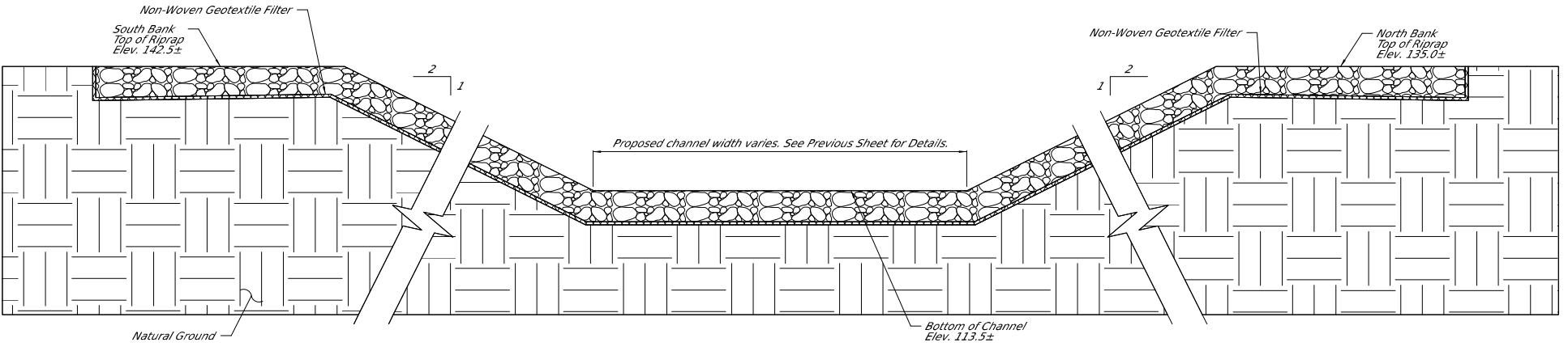
SECTION C-C Proposed Channel Typical Section Looking Downstation
