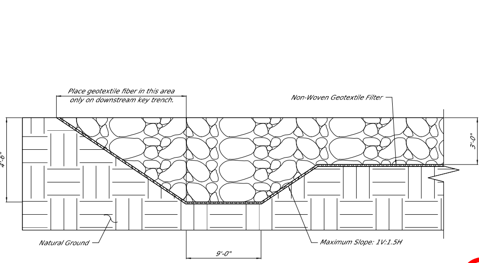
SECTION A-A Termination Key Trench Detail for Upstream & Downstream Termination Not to Scale
