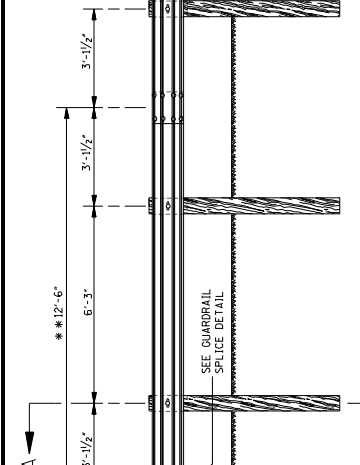
SECTION A-A DOUBLE-FACED BARRIER
