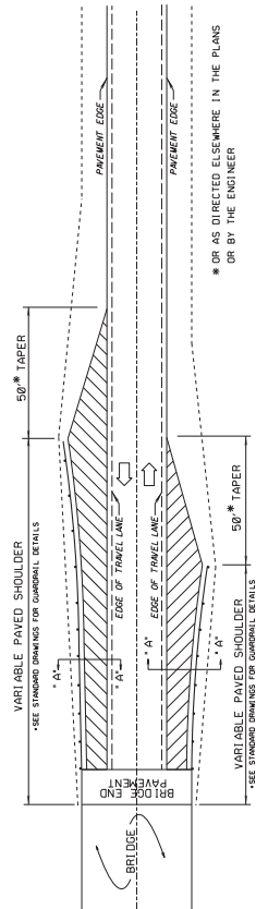
TYPICAL DETAIL OF PAVED SHOULDERS AT BRIDGE ENDS (2-WAY TRAFFIC) SEE SECTION A-A
