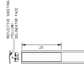
DETAIL OF TYPE I FLEXIBLE POST DELINEATOR
