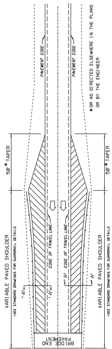
TYPICAL DETAIL OF PAVED SHOULDERS AT BRIDGE ENDS (1-WAY TRAFFIC)
