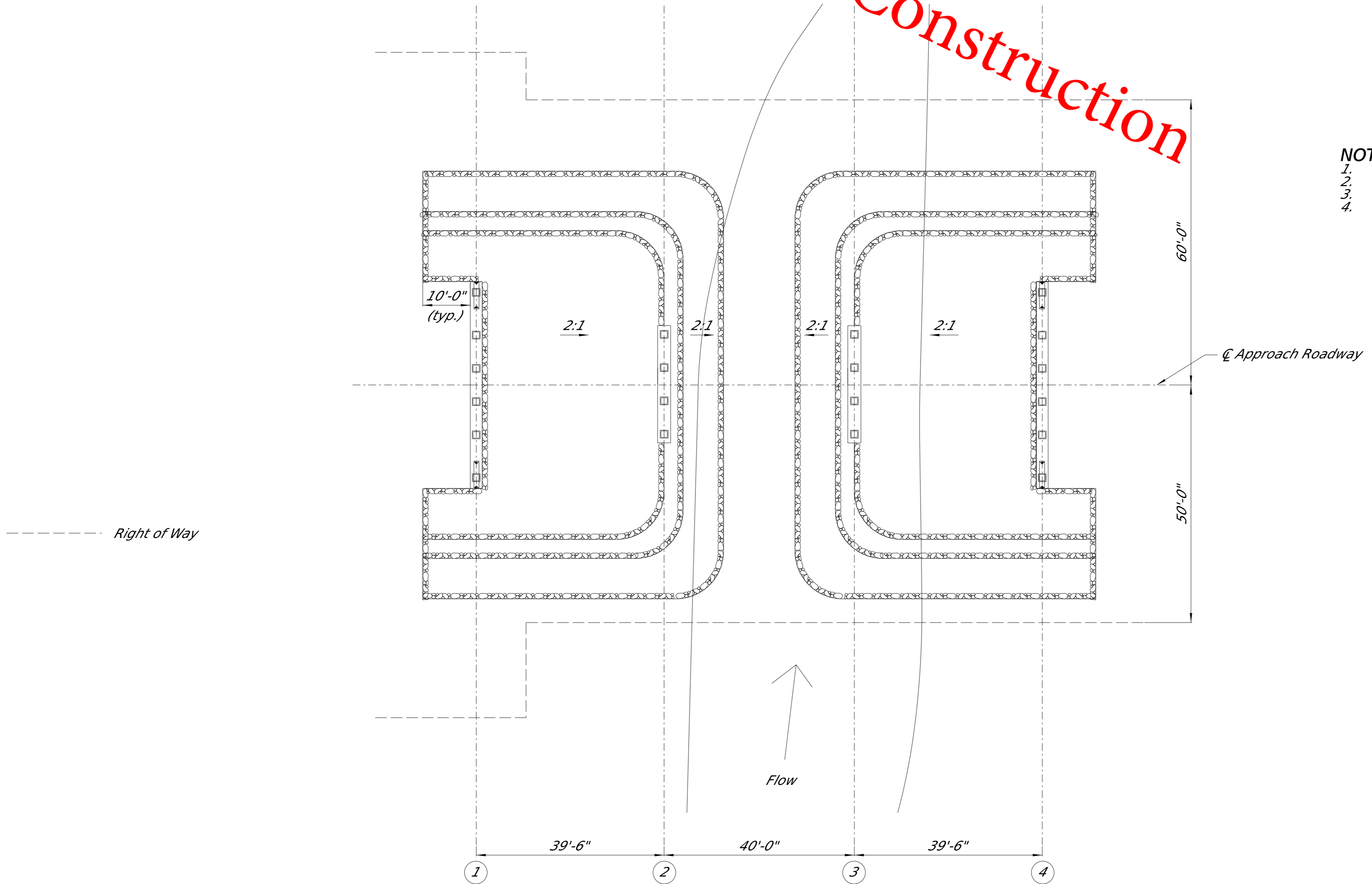
RIPRAP PLACEMENT PLAN
