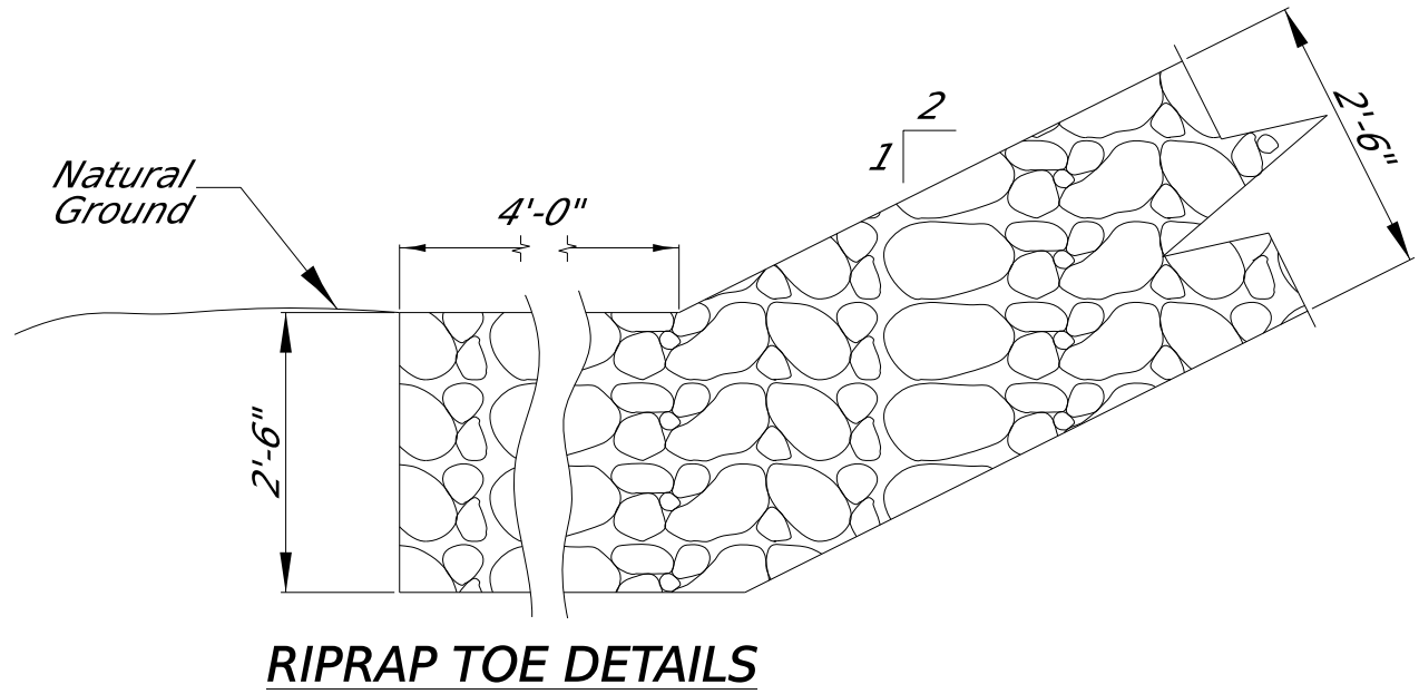
RIPRAP TOE DETAILS
