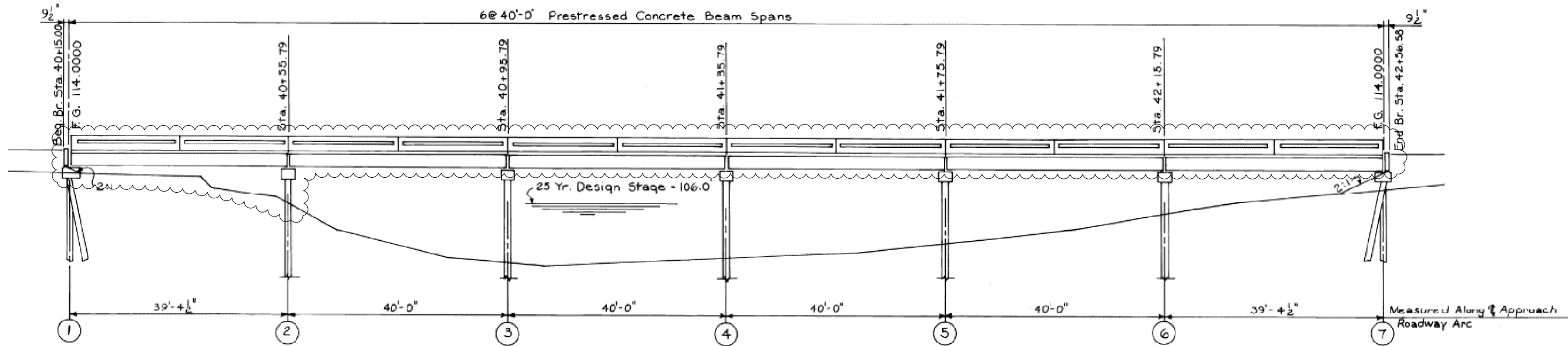
ELEVATION OF EXISTING BRIDGE (0.7)
