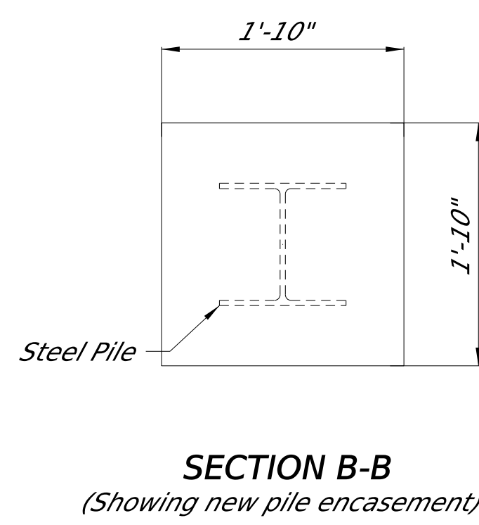
PILE ENCASEMENT DETAILS
