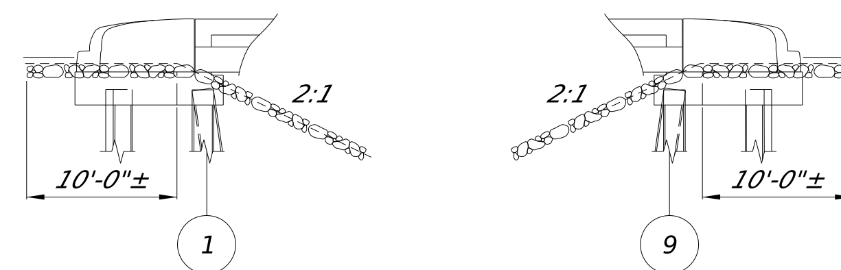
SR 438 RIPRAP PROFILE
