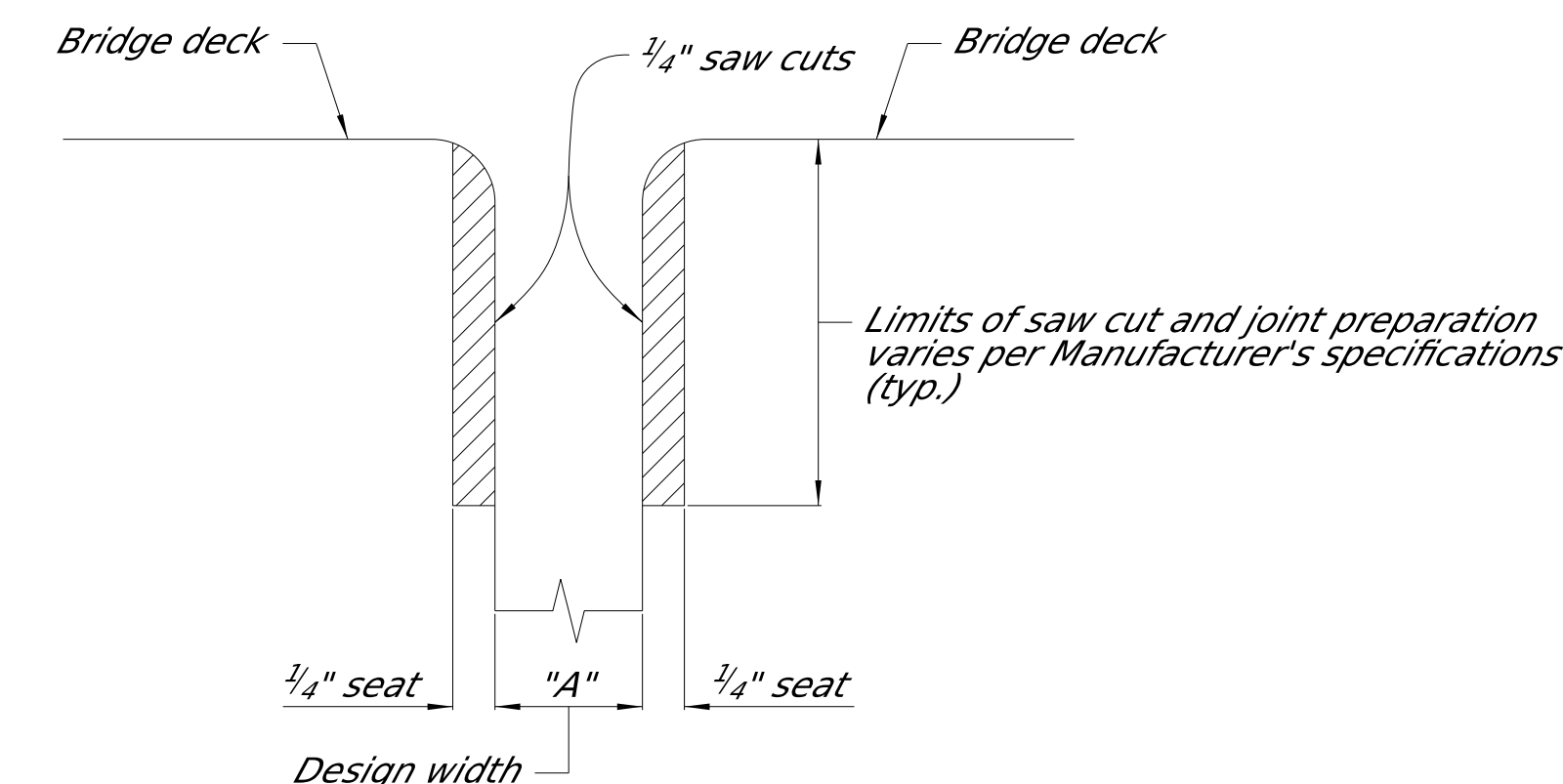
TYPICAL SECTION AT JOINT AFTER REMOVAL OF EXISTING SEAL AND SAW CUTS
