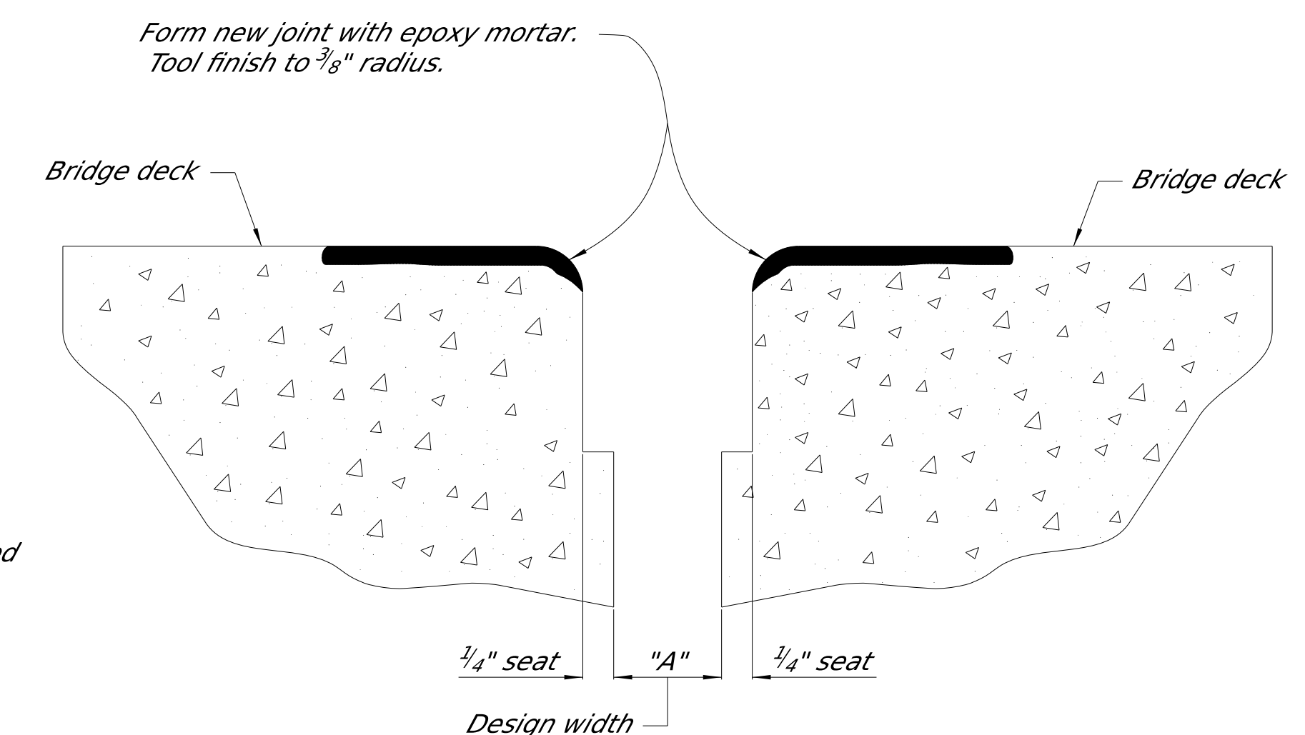
TYPICAL SECTION AT SAW CUTS & JOINT REPAIR
