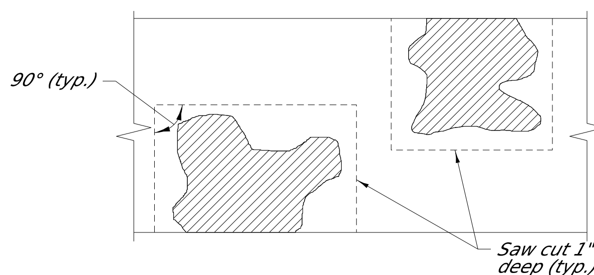
EPOXY REPAIR DETAILS
