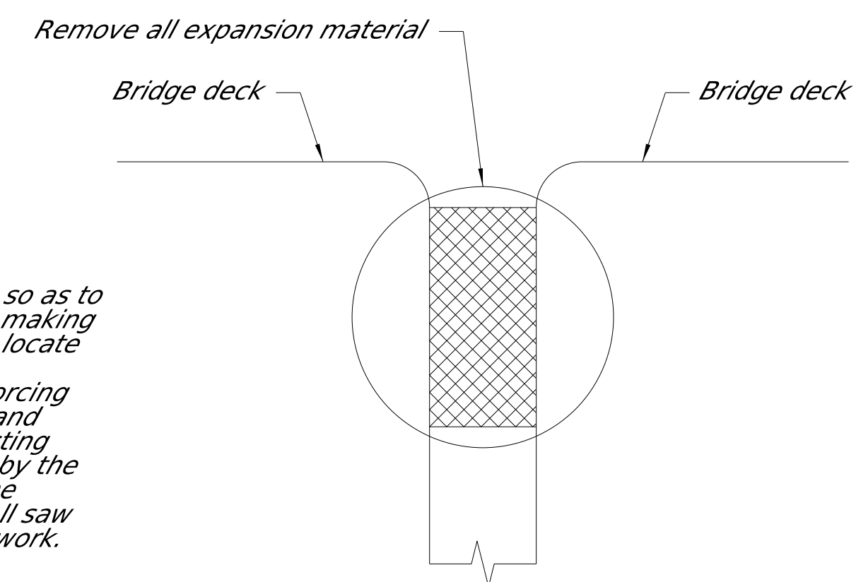
TYPICAL SECTION AT EXISTING JOINT
