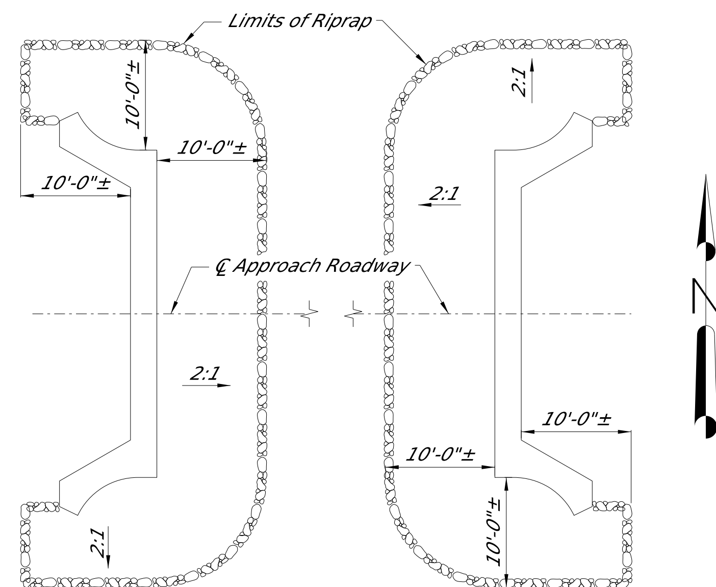
SR 438 RIPRAP PLAN
