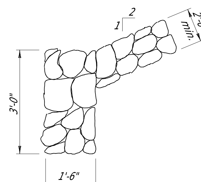
RIPRAP TOE DETAILS
