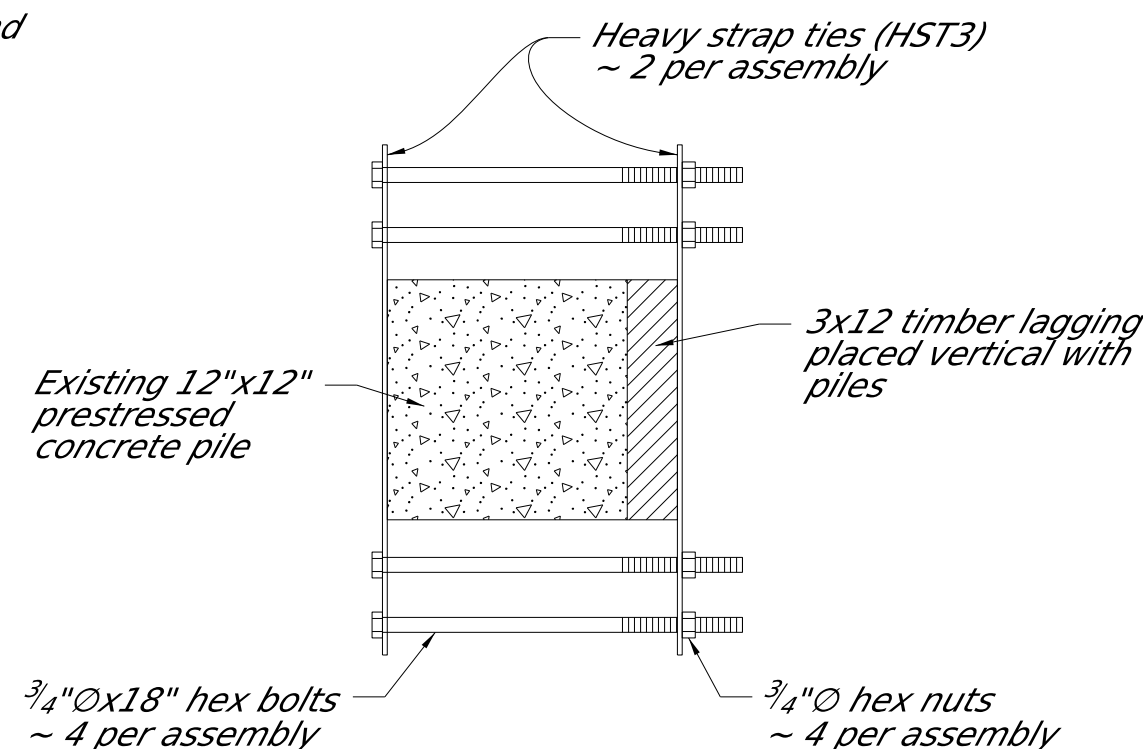
SECTION C-C
